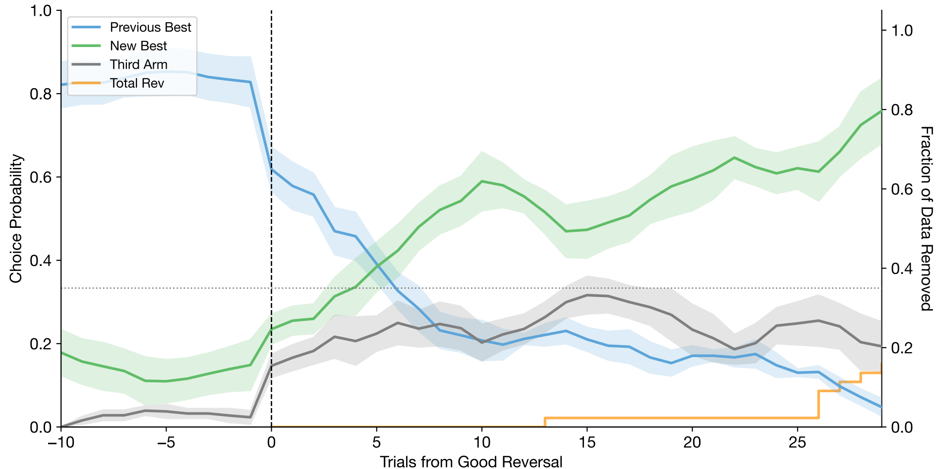
Good Reversal-Aligned Choices (mean \pm se across subjects | n=5 subjects, n=44 reversals)
